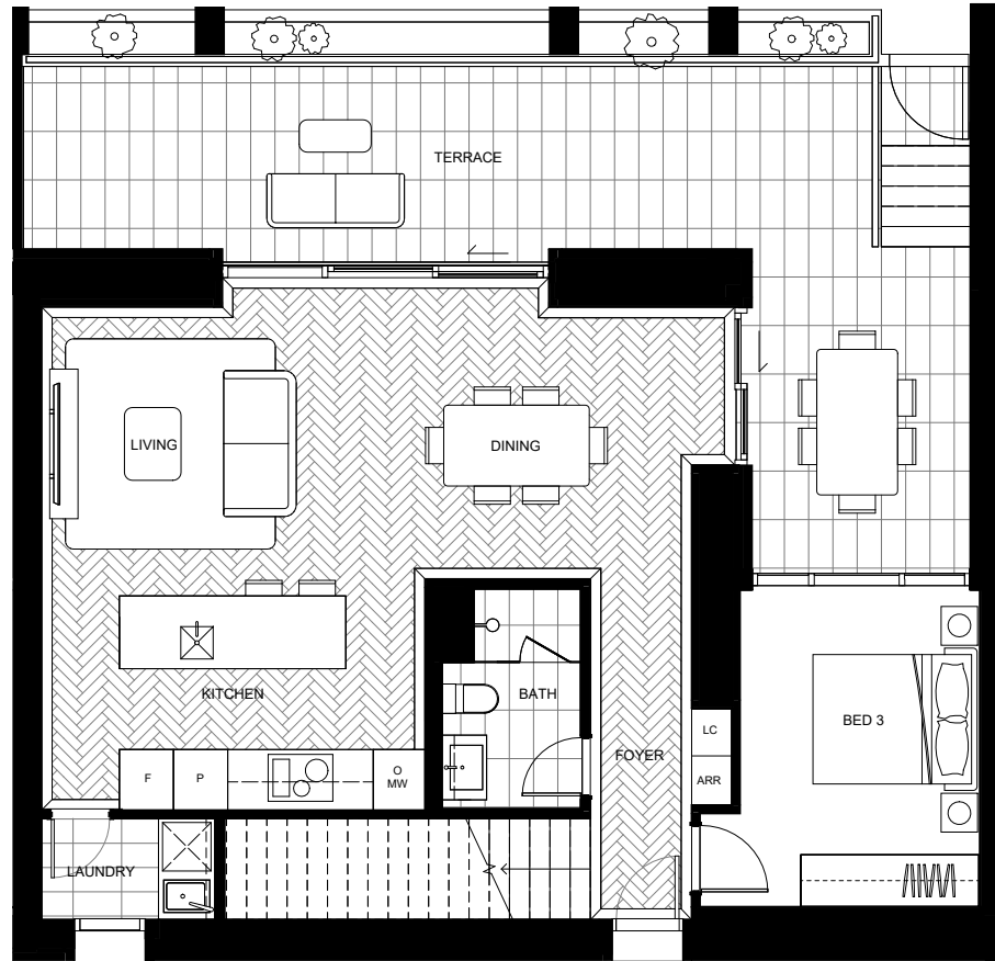
GROUND FLOOR / LEVEL 1
